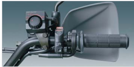
⑪ Grip Heater Kit ⑫ Sub Harness + & - Flexible, adjustable grip heater to warm fingers on cold winter mornings. The grip heater incorporates a plate that heats the underside of the grip. Integrated circuit to protect the battery from drain. For connection you should purchase item 11.
